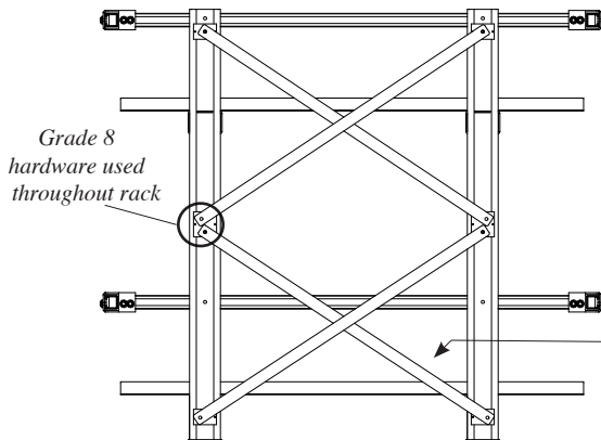
Side View of 2 tier, single row rack
