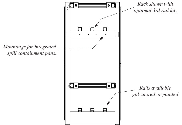
End View of 2 tier, single row rack
